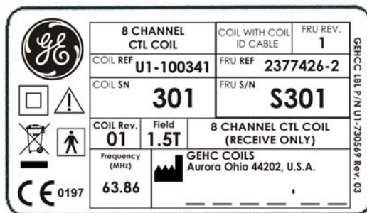
Figure 1: Coil label.
